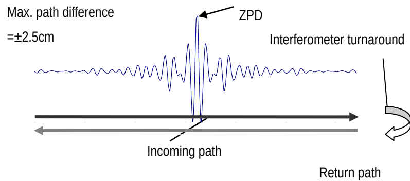
Figure A.2-3 Scanning by the Fourier interferometer
