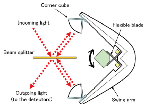
Figure A.2-4 Layout of the double corner cubes, swing arm and flexible blades
